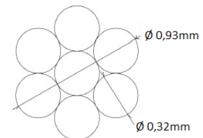
Sealing Wire Dimensions
